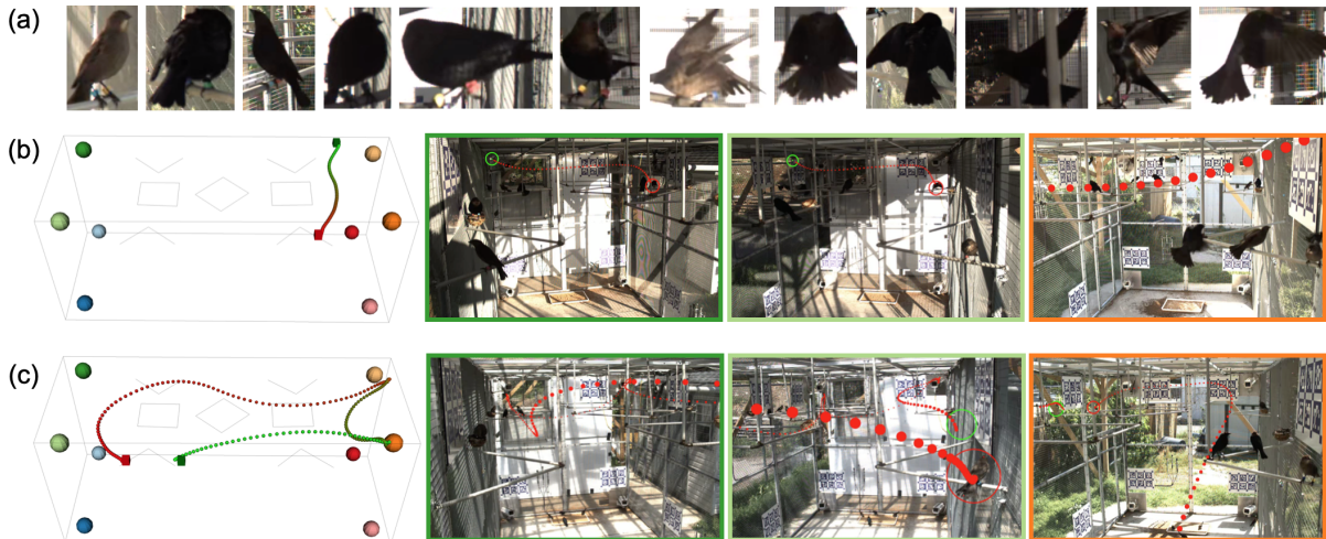
Fig. 4: Qualitative tracking results. (a) Examples of detected bird instances with variations in pose, shape, lighting, scale, occlusion, and motion blur. (b) Example of a successful short track (56 frames) followed by its 2D projections in 3 different views. Colors indicating the camera views are consistent with those in Figure 3. The green cube/circle is the start 3D/2D position and the red cube/circle is the end position. Dots in the 2D images are smaller/larger as the bird gets further away/closer. (c) Example of a successful long track (375 frames). During flight, the individual hops on the wall and briefly pauses for 1-2 seconds. Examples in (b) and (c) are from video segments drawn from different days, demonstrating variable time of day and lighting.
