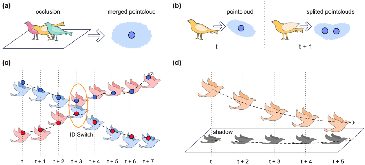
Fig. 5: Failure cases. (a) Inseparable pointcloud due to occlusions. (b) Merged/split clusters due to shape change of an individual at different instants of time, which could result in ghost trajectories. (c) Identity Switch. At first, the blue hypothesis is correctly tracking the ground truth blue bird. After a few frames, though, the blue bird and the red bird cross paths and blue hypothesis follows the wrong target. (d) Ghost trajectory resulting from false positive detections, eg. shadows of a bird.
