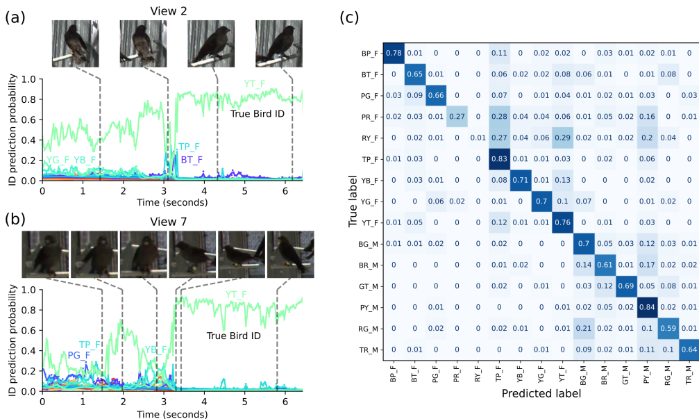
Fig. 6: Bird re-identification. We use a ResNet50 network supervised with triplet and ID losses to predict the identity of perched birds. In an example from the Bird15 test, a female with Yellow+Teal leg bands is visible from views 2 (a) and 7 (b). From view 2 (a) only its left leg band is initially visible, but the network has learned other features (such as tail shape, or background features if the bird is in a repeatedly used location) that allow it to correctly predict the identity. When no bands are visible (second image from the left in a), the confidence decreases. Once both bands are visible (third and fourth images) confidence increases again. From another view (b), both bands are visible, but are in a shadow and some initial color distortion causes the network to incorrectly predict Pink+Green, Teal+Pink, and Yellow+Blue, albeit with low confidence. As the bird reorients to face the other direction, both bands become visible with better lighting and confidence increases. A normalized confusion matrix (c) shows most birds are correctly identified 60–80% of the time in the test set. Increasing the detection confidence threshold from 0 to 0.8 improves accuracy from 0.68 to 0.97 while still correctly identifying 52% of the examples in the Bird15 test set.
