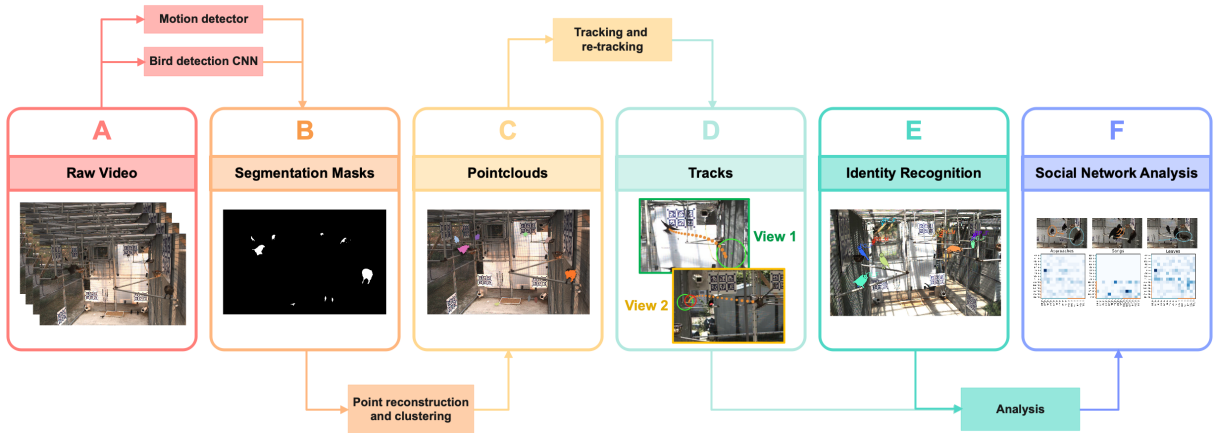
Fig. 1: Full pipeline for cowbird tracking and recognition. (A) A synchronized set of raw videos from multiple views are processed in a frame-by-frame manner. (B) Segmentation masks of bird instances are obtained using a Mask R-CNN network and background subtraction. (C) Pointclouds are reconstructed by multi-view matching, triangulation, and clustering. (D) Tracking, which is implemented using a Lagrangian Particle Tracking (LPT) algorithm, links pointclouds in time to form tracklets. Re-tracking associate 3D tracklets to generate longer 3D tracks. (E) Individual identity recognition using the FastReID framework. (F) Output from the pipeline can then be used for social network analysis.
